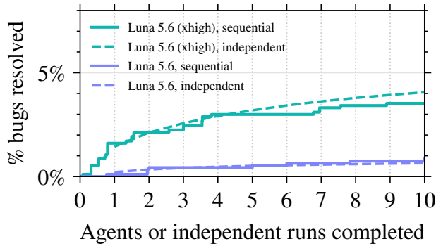
Figure 7 Repeated attempts fix additional bugs, but gains diminish. Results on the 5 repositories with the most bugs. Solid curves show sequential agent runs, each starting from the preceding agent’s patch while dashed curves show the union of bugs resolved by independent attempts.
