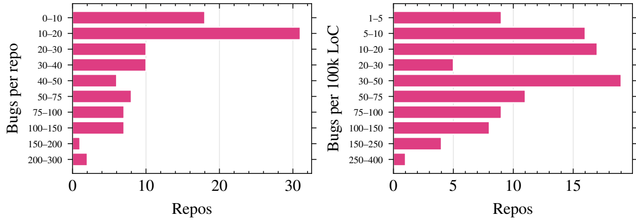
Figure 22 Binned repository-level distributions.
