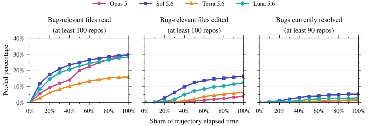
Figure 19 The same reading, editing, and resolved-bug results with progress measured by elapsed time. Progress is from 0% to 100% within each run. Repository counts report how many runs have available time and hidden-test results. We do not count missing results as failures.
