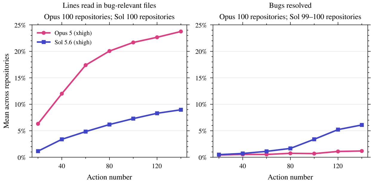
Figure 21 Lines read in bug-relevant files and bugs resolved by action number for Opus and Sol. Each result is the mean across repositories. Lines are included only for reads with exact line ranges. Bug resolution is from the most recent evaluated patch.
