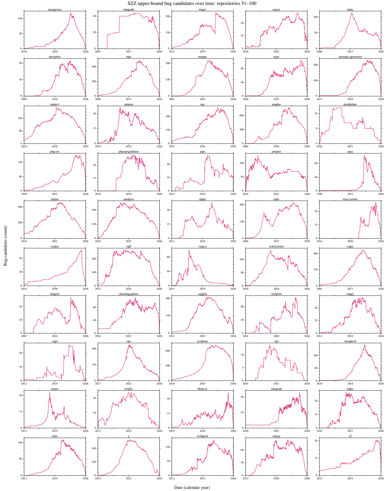
Figure 26 Estimates of the number of concurrent bug instance candidates across the histories of benchmark repositories 51–100, in the order listed in Table 29.
