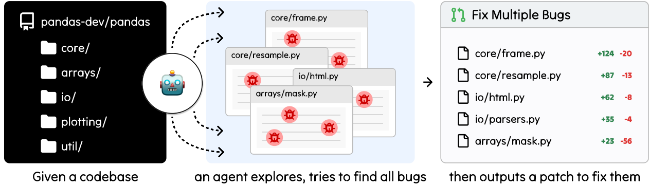
Figure 1 SWE-sweep evaluates coding agents on their ability to identify and fix unspecified bugs within a software repository. An agent is asked to scour a codebase for issues and resolve them without any information about specific faults. The agent is then graded using a suite of hidden tests.
