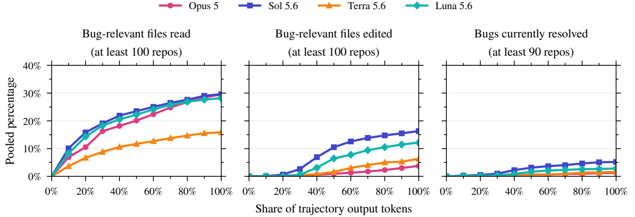
Figure 18 The same reading, editing, and resolved-bug results with progress measured by output tokens. Progress is from 0% to 100% for every run. Reading changes after each action; editing and resolution change only when a patch is evaluated. We do not count missing hidden-test results as failures.
