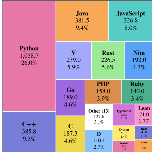
Figure 3 Bug counts and ratios by language, measured from the files modified by gold fixes. Details in Table 28.
