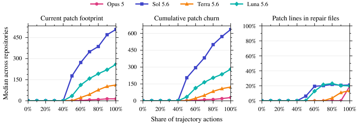
Figure 20 Patch changes over the percentage of actions in each run. The first result shows the number of lines changed in the current patch. The second shows all line changes from one patch to the next across the run. The third shows the percentage of current changed lines in bug-relevant files. Each result is the median across 100 repositories. At 100%, the patch is the submitted patch.
