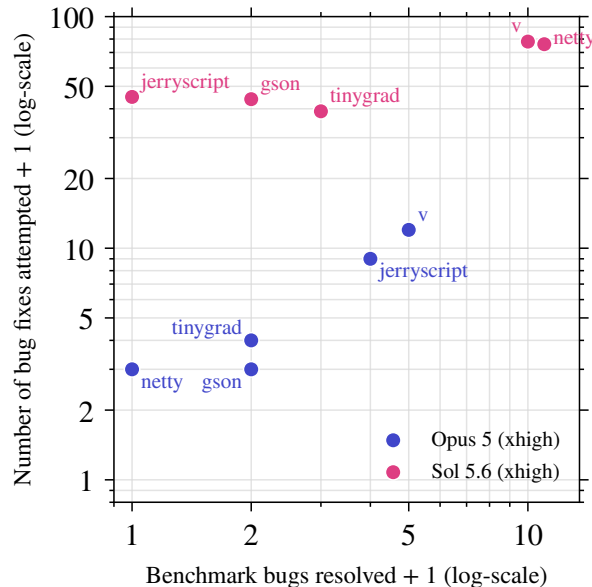
Figure 11 Benchmark bugs resolved and bug fixes attempted for several repositories.
