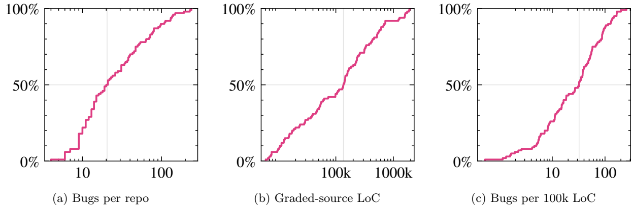
Figure 23 Empirical cumulative distributions of repository-level benchmark statistics. Faint-gray guides mark the median value and 50th percentile.
