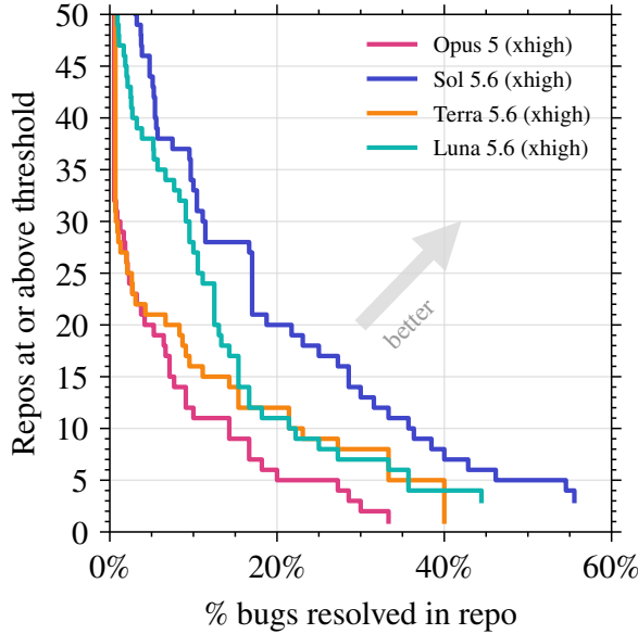
Figure 5 Distribution of repository-level bug-resolution scores. The endpoint of each line indicates the best repository-level score.
