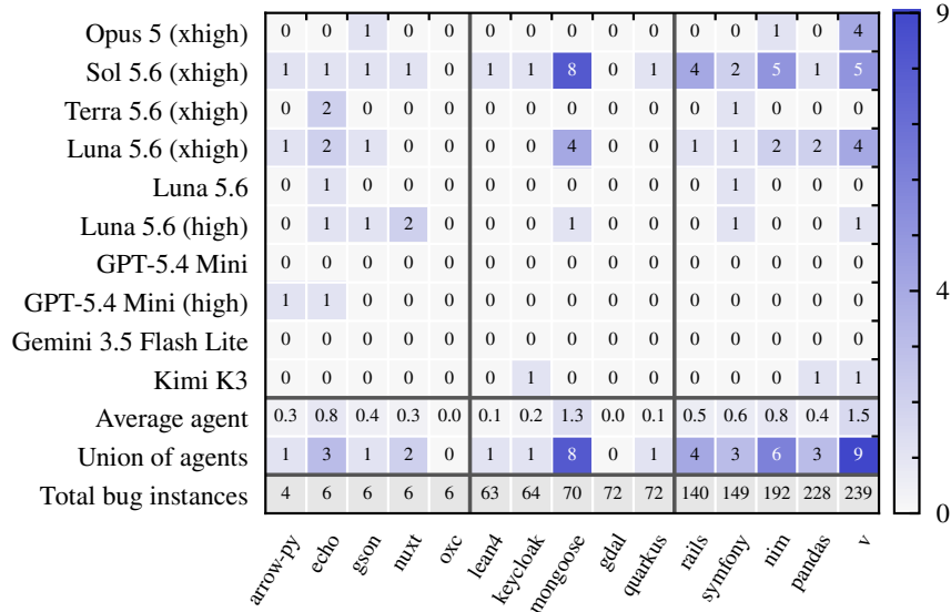
Figure 15 Number of bugs resolved for the five smallest repositories below 25 benchmark bugs, the five largest repositories with 25–74 bugs, and the five largest repositories with at least 75 bugs. Average agent is the mean across models; union of agents counts distinct bugs resolved by at least one model. The final row gives each repository’s total benchmark bug instances.
