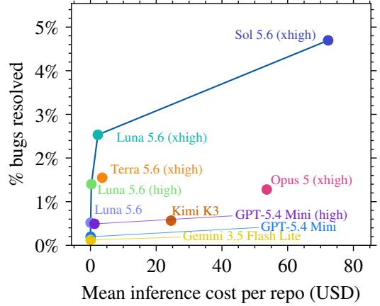
Figure 4 Bugs resolved versus inference cost; the line marks the Pareto frontier.
