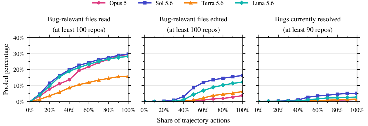
Figure 17 Bug-relevant files read, bug-relevant files edited, and bugs resolved over the percentage of actions in each run. All three results use the same range from 0 to 40%. Each curve is the percentage across all bugs in all repositories. Reading changes after each action; editing and resolution change only when a patch is evaluated. We do not count missing hidden-test results as failures.
