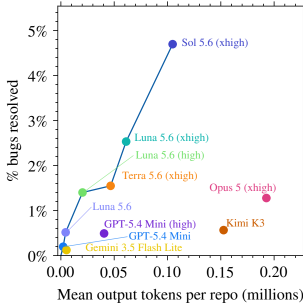
Figure 14 Percentage of bugs resolved versus mean total output tokens per repository; the line marks the Pareto frontier.
