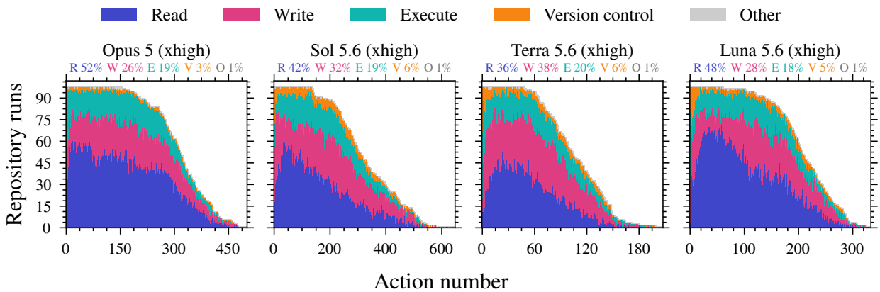
Figure 16 Distribution of observable actions for each model across 100 repositories. Actions are ordered from the start to the end of each run. At every action number, the figure shows the number of runs with a read, write, execute, version-control, or other action. Not every run is present at later actions because runs use different numbers of actions; the number does not measure performance. Labels show the percentage across all actions.
