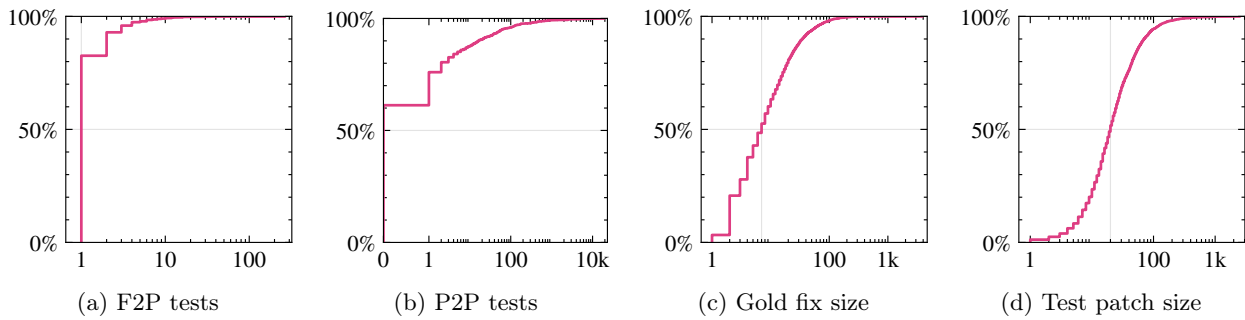
Figure 24 Empirical cumulative distributions of bug-level benchmark statistics. Faint-gray guides mark the median value and 50th percentile.
