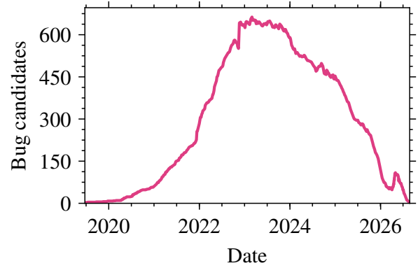
Figure 13 Number of concurrent bug instance candidates across the history of V.
