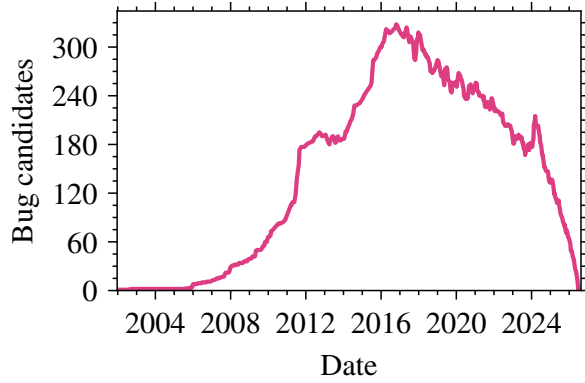
Figure 12 Number of concurrent bug instance candidates across the history of NumPy.
