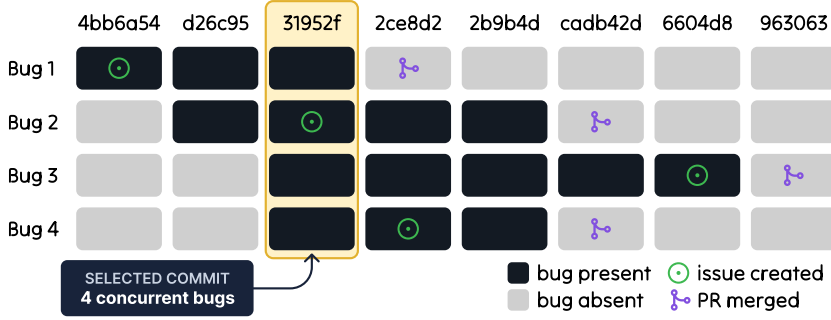
Figure 2 SWE-sweep tasks are constructed from a repository’s buggiest commit. Rows represent bugs, columns are commits; dark cells indicate a bug is present at a commit. The 31952f codebase becomes the task start state ( base commit ).
