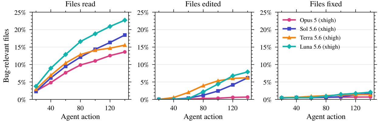
Figure 6 Agents reach far more bug-relevant files than they fully fix. We show every file changed by a gold fix and report whether each model has read or edited it and whether every bug whose gold fix changes that file is resolved. Read means an agent explicitly read the file; edited means an agent edited a file involved in a gold fix; a fixed file requires all accepted bugs related to the file to pass together at a checkpoint with no correctness test regression.
